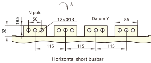
Horizontal short busbar
