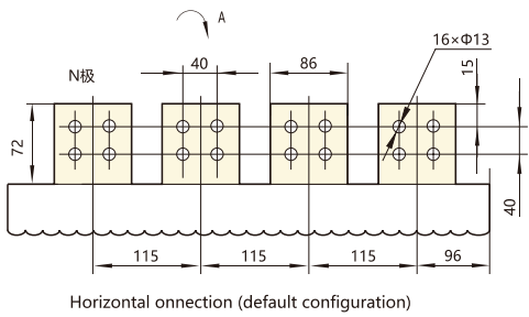
Horizontal onnection (default configuration)
